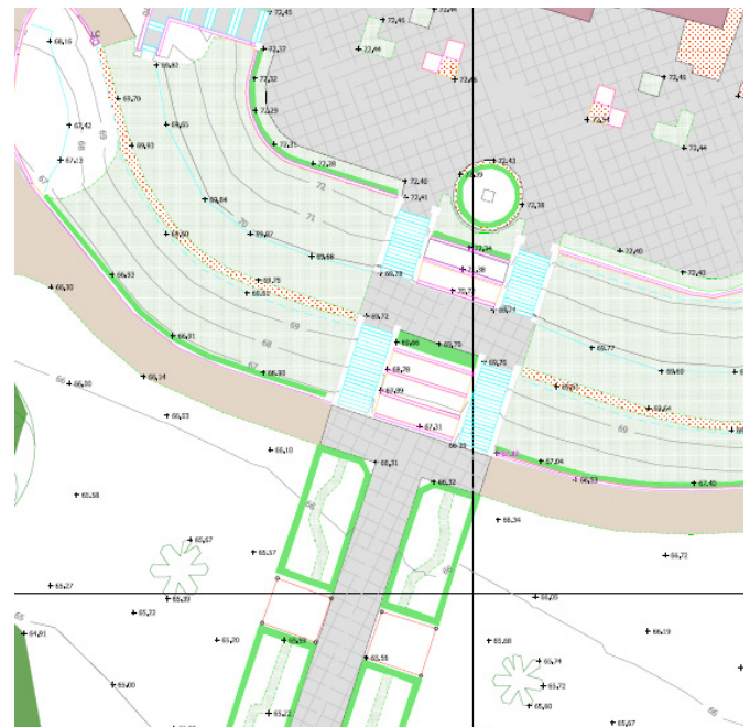
Conventional survey of a re-development site
